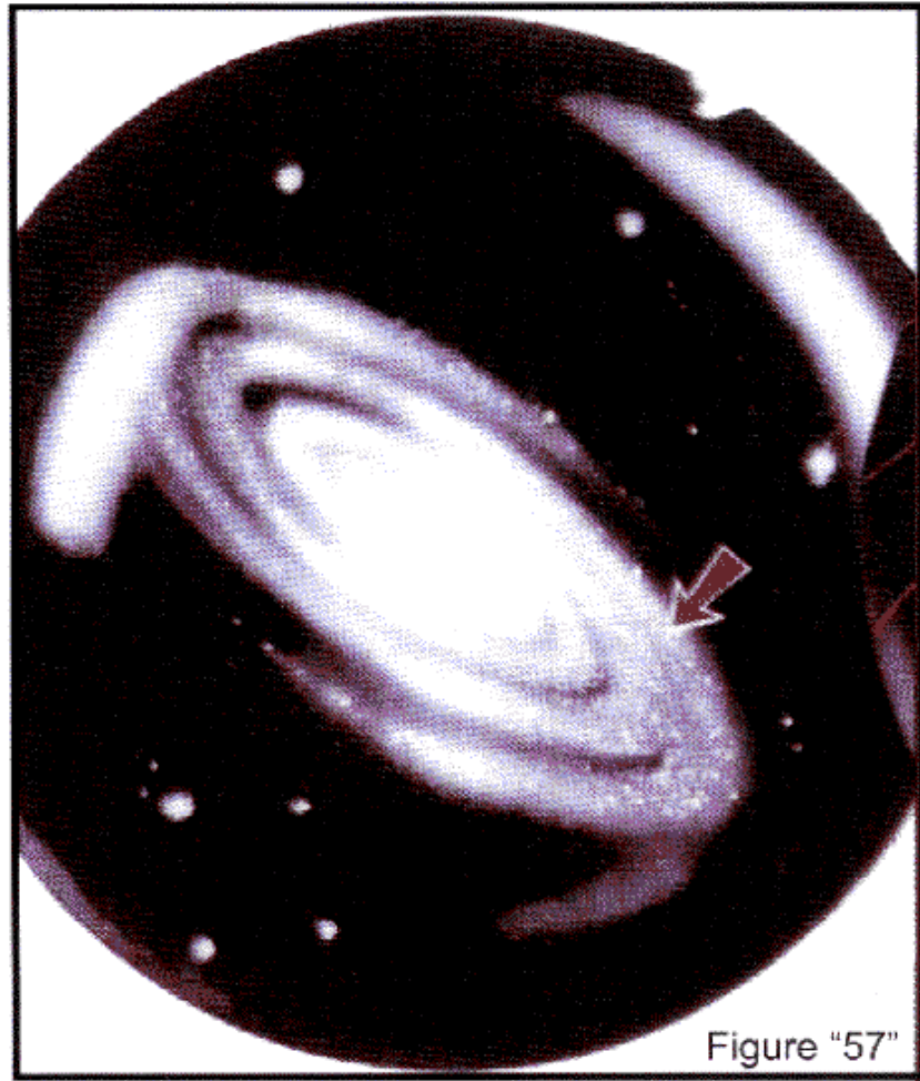
The arrow points to the place of our solar system in our galaxy, our world being just a particle of dust in it.
