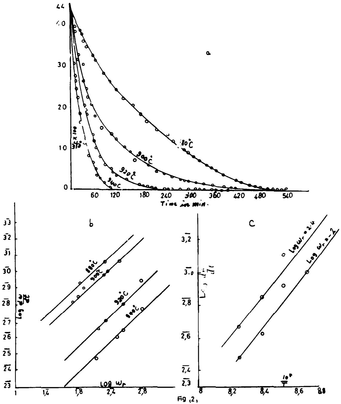
Fig.(2) Treatment (a) shows the relation between \frac{w_0 - w}{w_0} \times 100 and time (t). treatment (b) shows the relation between \log \frac{dw}{dt} and \log w_r at constant temperatures 880°, 900°, 920° and 940°C. treatment (c) shows the relation between \log \frac{dw}{dt} and \frac{10^4}{T} for various values of \log w_r .
